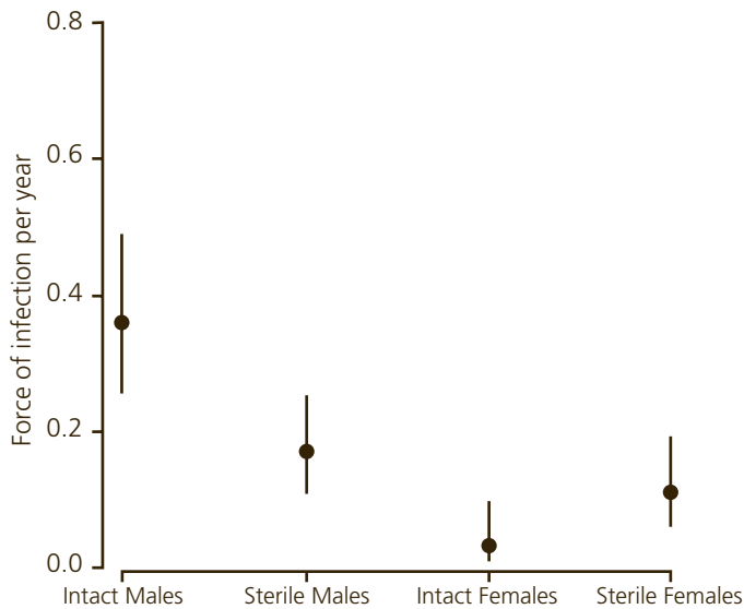
Fig. 2. Estimates of the force of infection ( \pm standard error) of M. bovis in intact and sterilised male and female possums.
