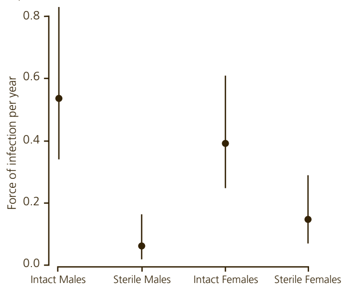
Fig. 1. Estimates of the force of infection ( \pm standard error) of L. balcanica in intact and sterilised male and female possums.
