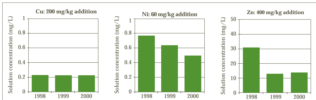
Figure 9. Soil solution Cu, Ni, and Zn concentrations in 1998, 1999, and 2000, after amendment at the highest metal addition levels. Note the change in scale for Zn.
