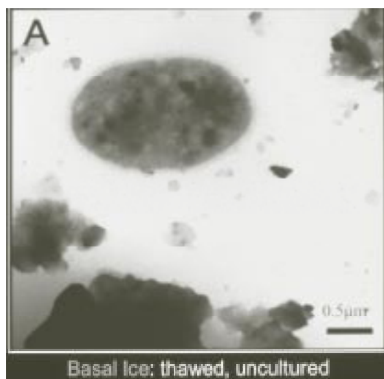
Figure 8. Transmission electron microscopy image of bacteria in glacial meltwater (scale bar is 0.5 microns)
