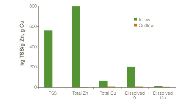
Figure 3: Mass of Total Suspended Sediment (kg of TSS), and total and dissolved zinc and copper (g of Zn and Cu) flowing into, and discharged from the raingarden during five Spring events in 2006
