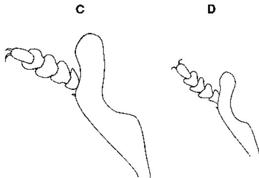
Fig. C, D Right front tibia and tarsus, male, Chaerodes trachyscelides and C. laetus (spines and setae omitted).
