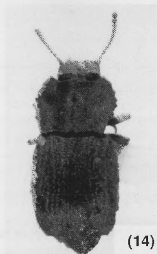
Fig. 11–19 Lagriinae, Adellini: (11) Edalrus curtulus , Waipoua S.F., ND. (12) Exadelium rufilabrum , Dun Mntn, NN. (13) Kaszabadelium aucklandicum , Pouakai Ra., TK. (14) Mesopatrum granulatum , Marlborough, MB. (15) Mitua triangularis , Puketū State Forest, ND. (16) Periatrum rotundatum , Wangapeka, NN. (17) Stenadelium striatum , Kaweka Ra., HB. (18) Zeadelium parvum , Table Hill, SI. (19) Z. senile , Coronet Pk, OL.
