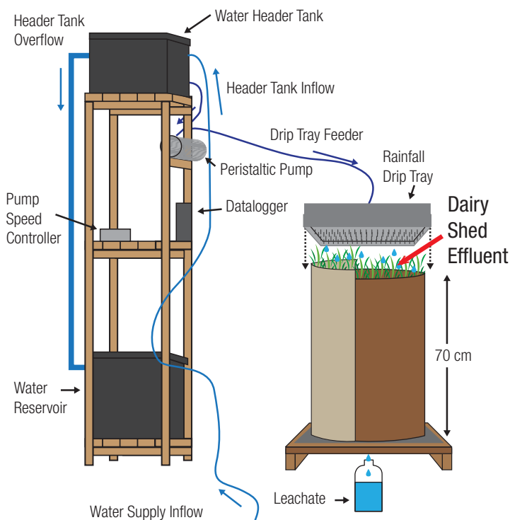
FIGURE 2 Experimental set-up.
