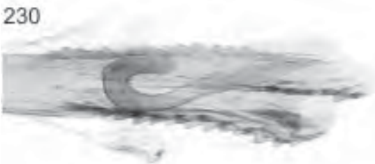
(222–231) Izatha , male genitalia, apex of phallus (selected species): 222 I. attactella ; 223 I. blepharidota ; 224 I. voluptuosa ; 225 I. austera ; 226 I. copiosella ; 227 I. walkerae ; 228 I. mira ; 229 I. notodoxa ; 230 I. katadiktya ; 231 I. apodoxa (N.B., fishhook cornutus broken; 3 rd toothed ridge distinguishing this species from notodoxa arrowed).
