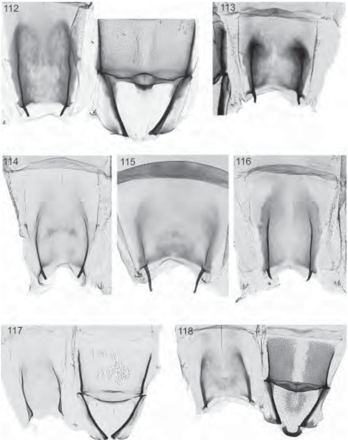
Fig. 112–118 Izatha , adult abdominal base, descaled: (112) I. attackella male, S2 and T1–2; (113) I. mira male, S2; (114) I. apodoxa male, S2; (115) I. balanophora female, S2; (116) I. peroneanella male, S2; (117) I. oleariae male, S2 and T1–2; (118) I. prasophyta male, S2 and T1–2. (Automontage photographs by R. J. B. Hoare and B. E. Rhode.)
