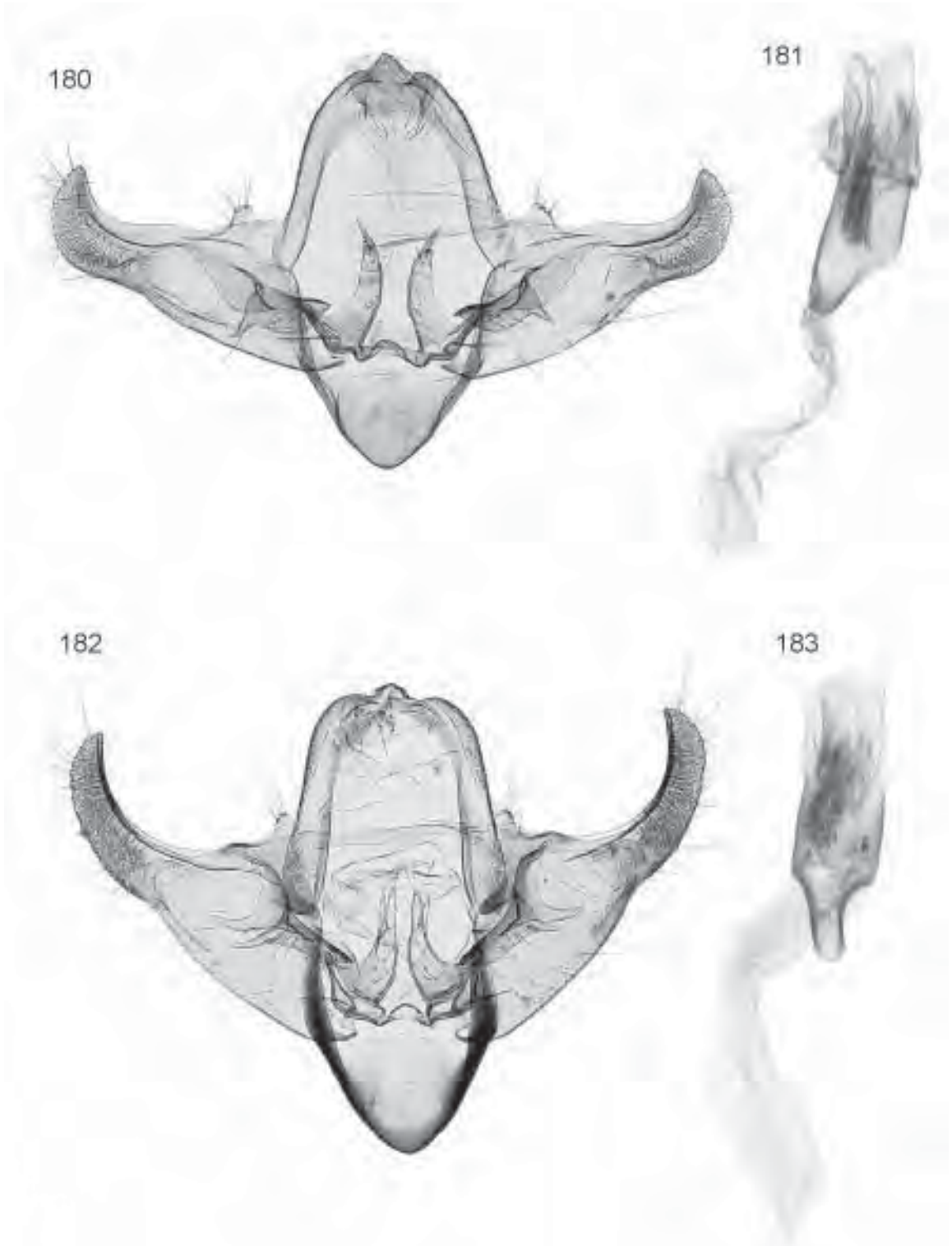
Male genitalia. (180, 181) Izatha huttonii : 180 genital capsule, 181 phallus (unmated specimen). (182, 183) Izatha peroneanella : 182 genital capsule, 183 phallus (unmated specimen).
