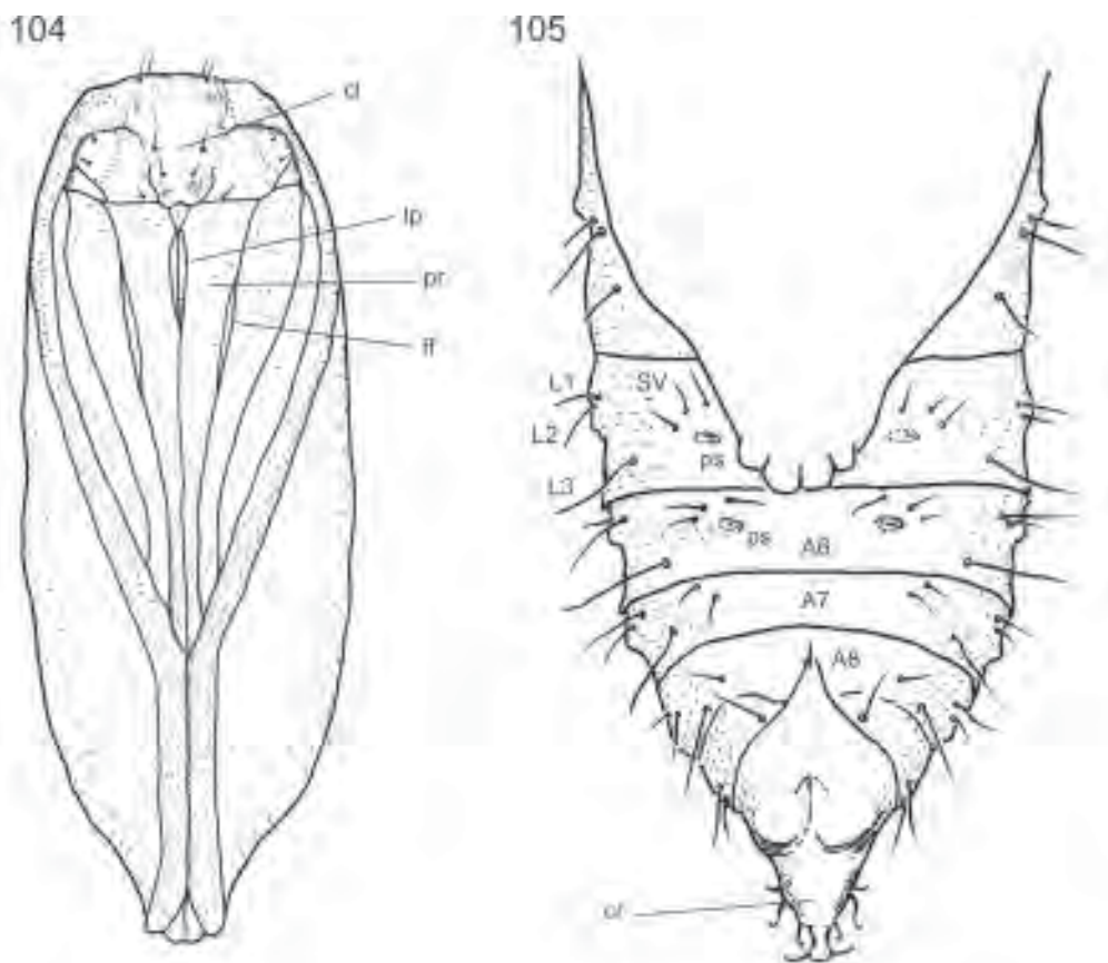
Fig. 104, 105 Pupa, Izatha oleariae , ventral view: (104) head, thorax; (105) A4–10. (cl, clypeus; cr, cremaster; ff, fore-femur; lp, labial palpi; pr, proboscis; ps, proleg scar.)
