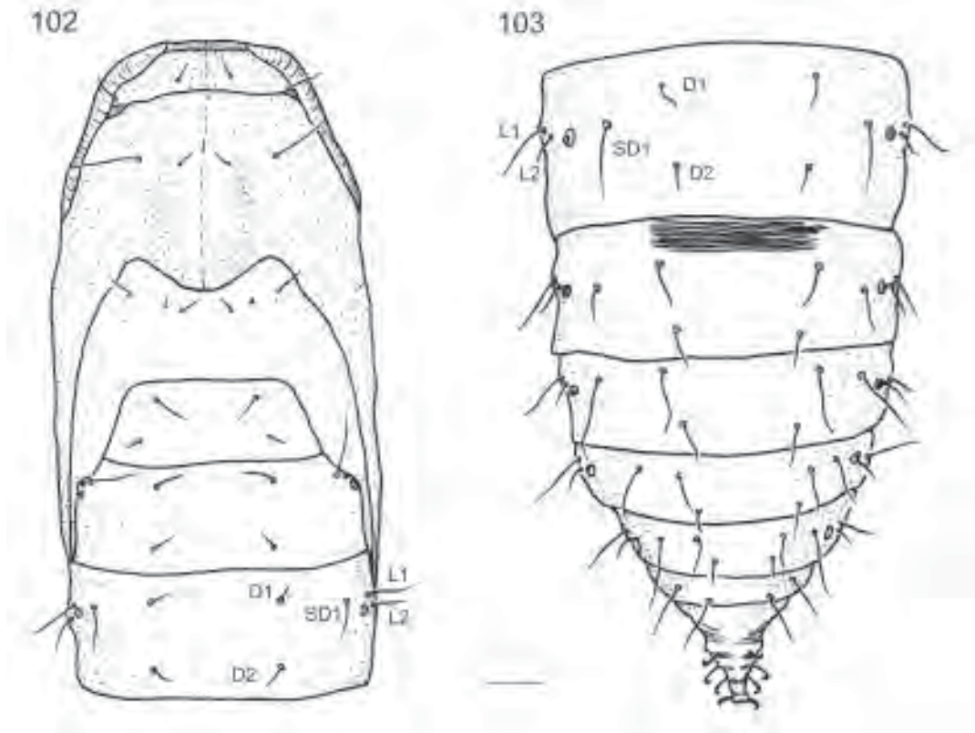
Fig. 102, 103 Pupa, Izatha oleariae , dorsal view: (102) head, thorax, A1-3; (103) A4-10.
