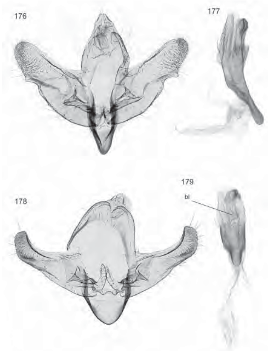
Male genitalia. (176, 177) Izatha heroica : 176 genital capsule, 177 phallus. (178, 179) Izatha hudsoni : 178 genital capsule, 179 phallus (mated specimen). (bl, basal flange of left lobe of phallus).
