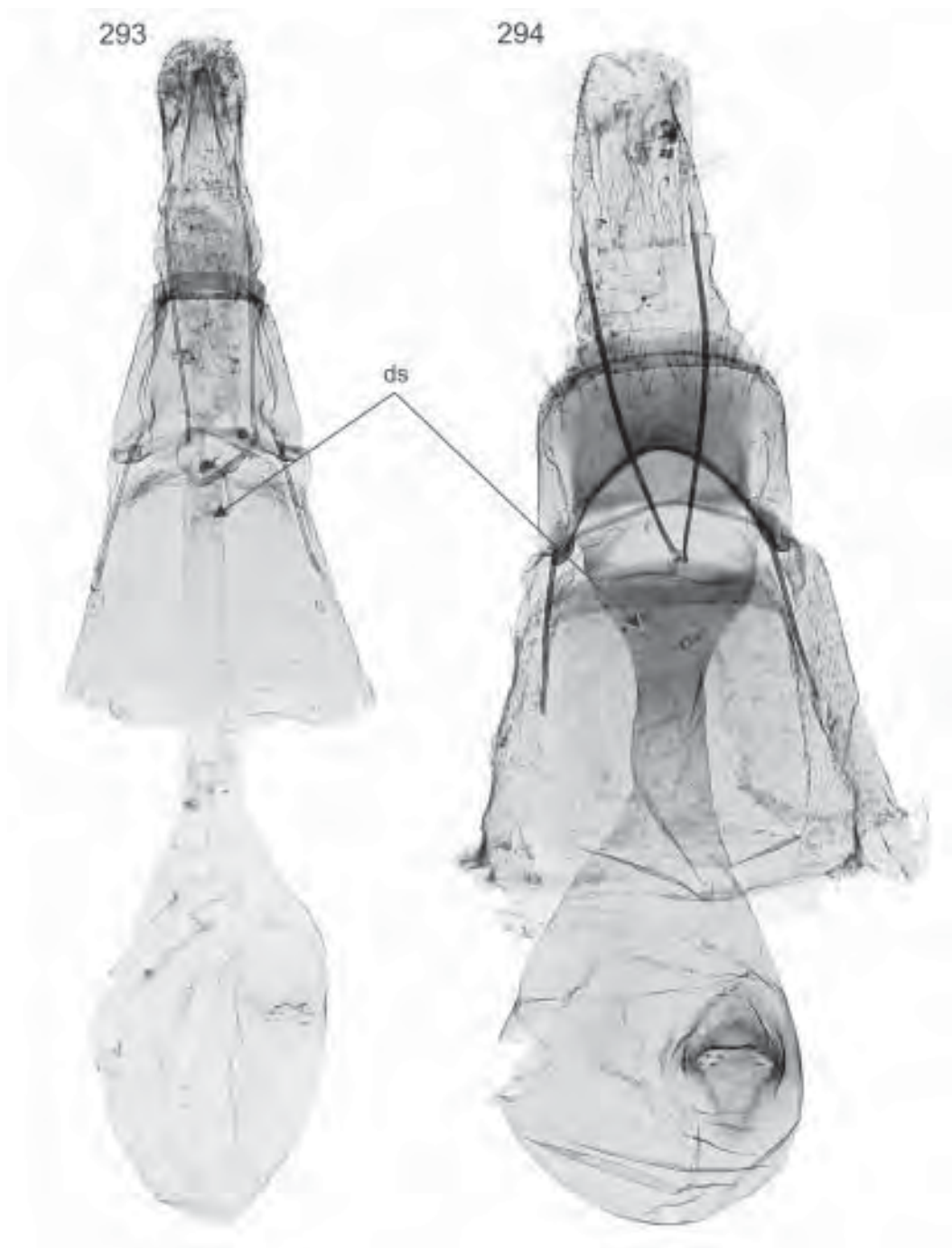
Female terminalia. (293) Izatha gibbsi ; (294) I. minimira . (ds, ductus seminalis inception.)
