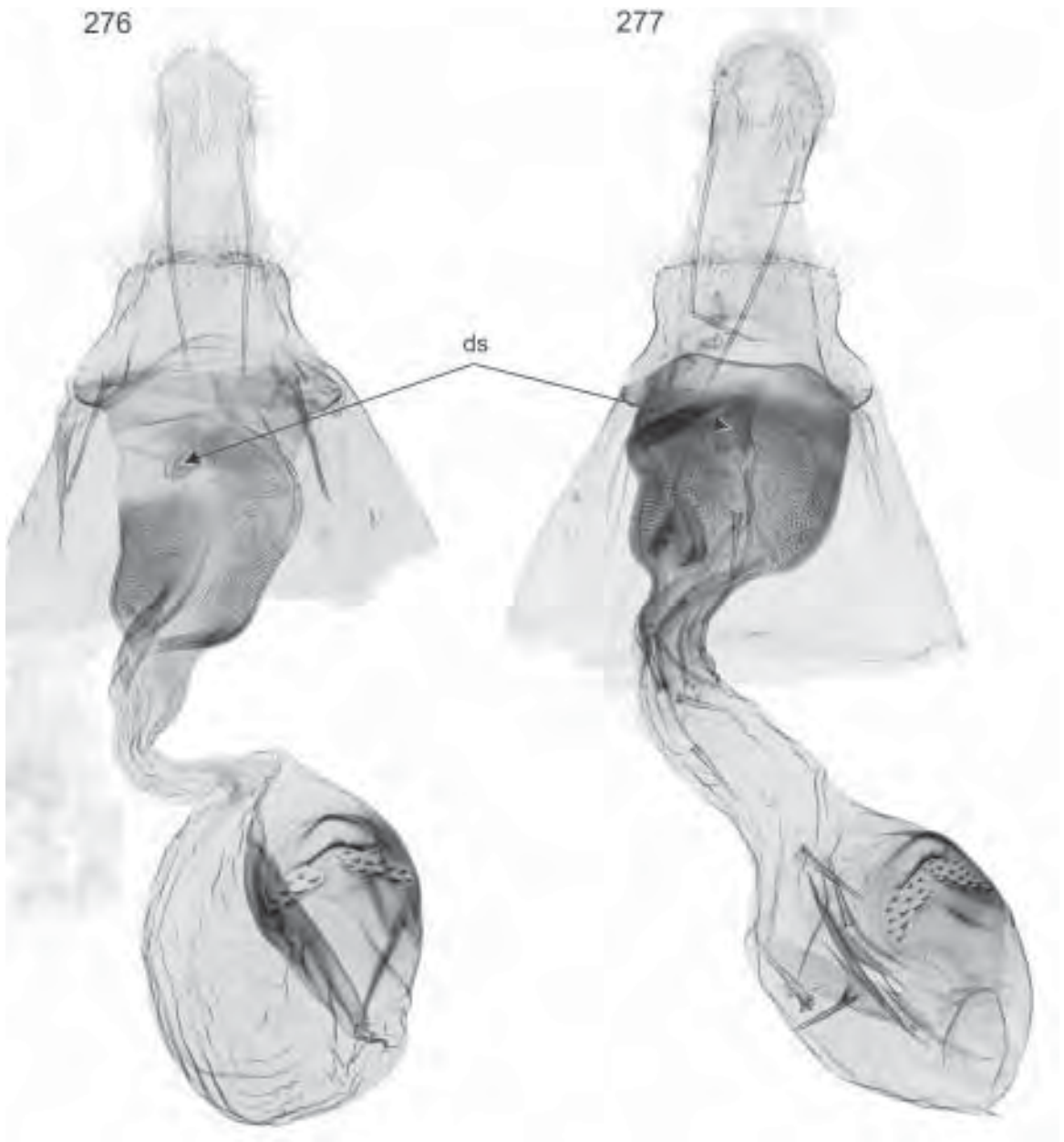
Female terminalia. (276) Izatha epiphanes ; (277) I. mesoschista . (ds, ductus seminalis inception.)
