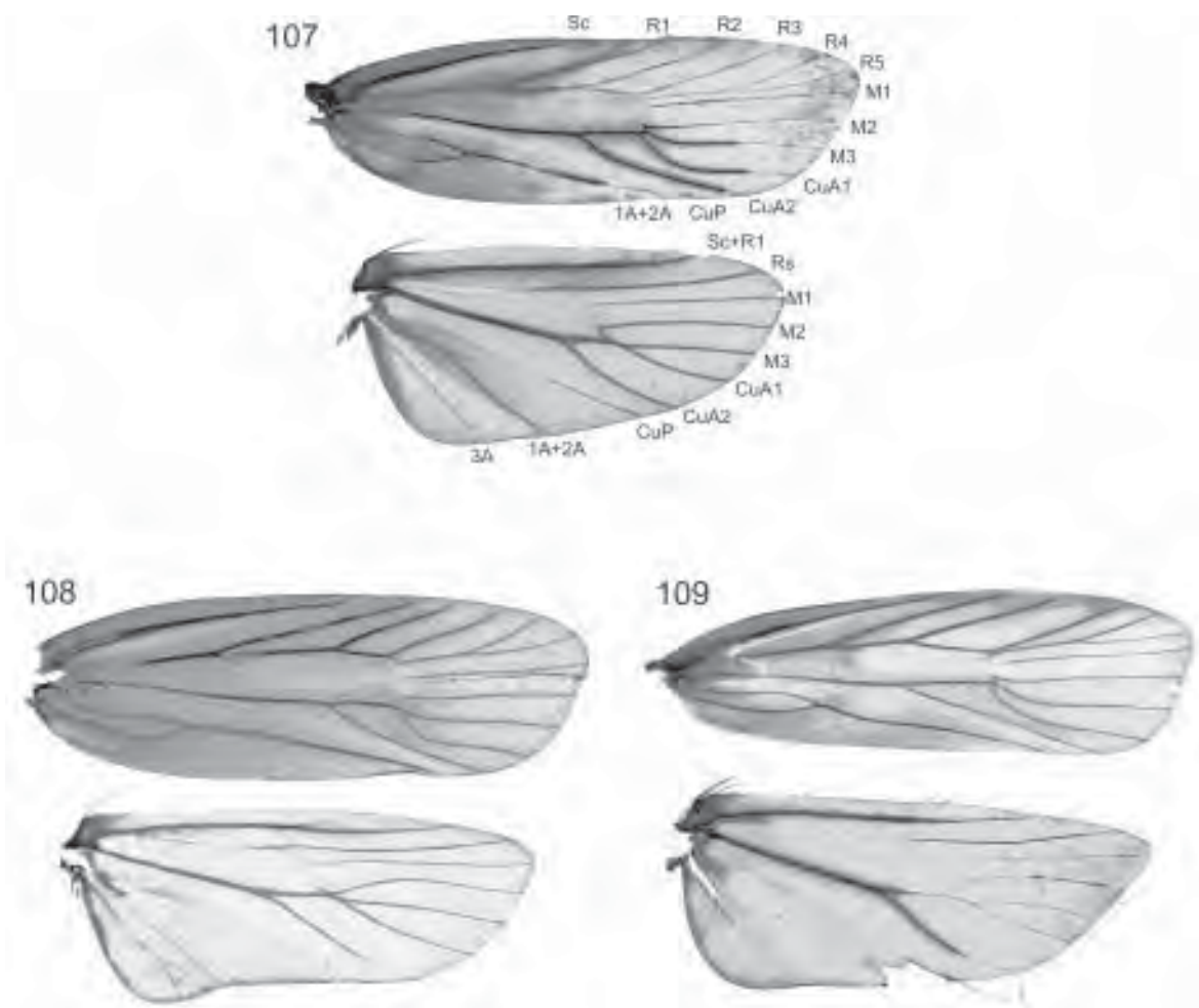
Fig. 107–109 Izatha , adult female wing venation: (107) I. mira ; (108) I. churtoni (note forked 3A of hindwing); (109) I. phaeoptila . (Automontage photographs by R. J. B. Hoare and B. E. Rhode.)
