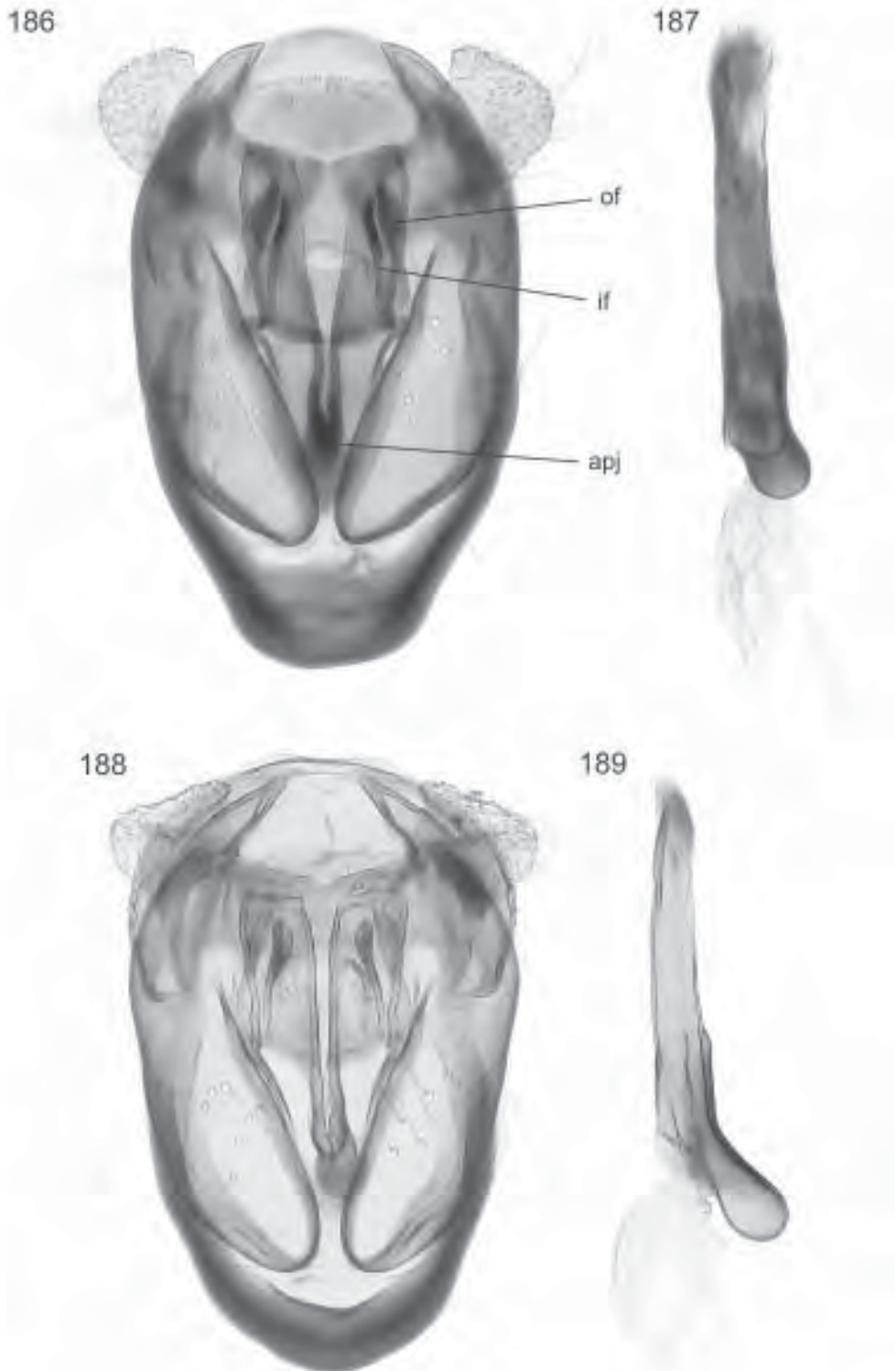
Male genitalia. (186, 187) Izatha oleariae : 186 genital capsule, 187 phallus. (apj, anterodorsal process of juxta; if, inner flange of juxta-costal plate; of, outer flange.) (188, 189) Izatha spheniscella : 188 genital capsule, 189 phallus.
