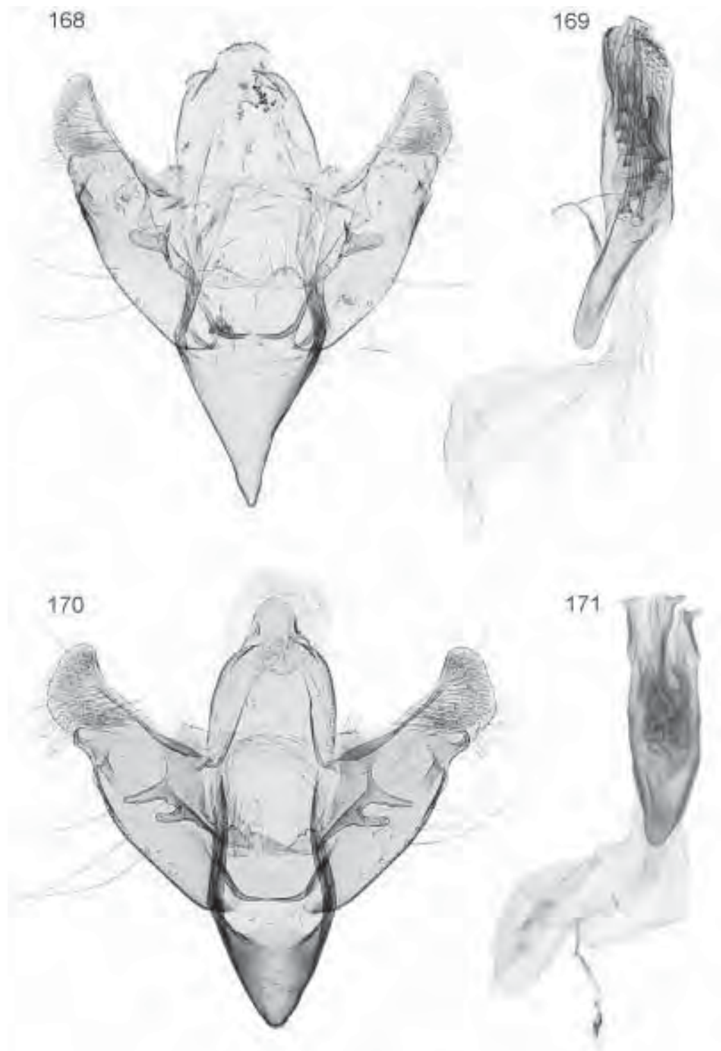
Male genitalia. (168, 169) Izatha epiphanes : 168 genital capsule, 169 phallus (unmated specimen). (170, 171) Izatha mesoschista : 170 genital capsule, 171 phallus (unmated specimen).
